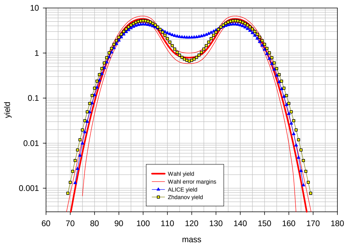
Benchmark B: ^{237}\text{Np} at 13 MeV, pre-neutron emission mass distribution
